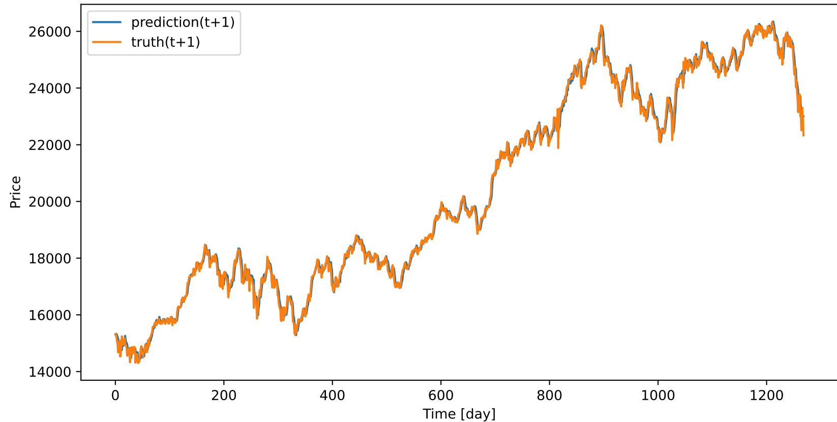
Test Set - Prediction vs Truth
